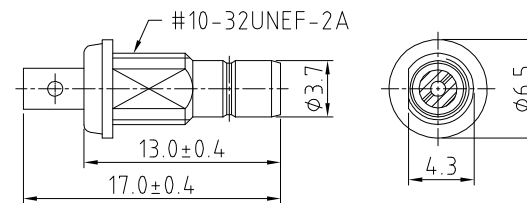
SMB JACK DETAIL DIMENSION
