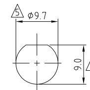
RECOMMENDED TNC MOUNTING HOLE
