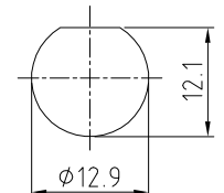
RECOMMENDED TNC MOUNTING HOLE
