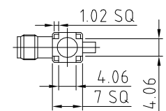
SMA JACK DETAIL DIMENSION
