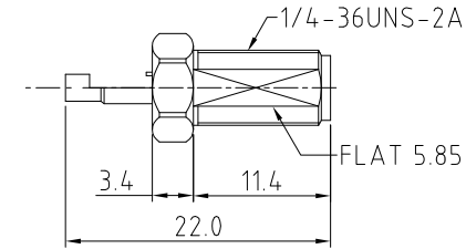
SMA JACK DETAIL DIMENSION
