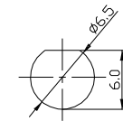
RECOMMENDED SMA MOUNTING HOLE
