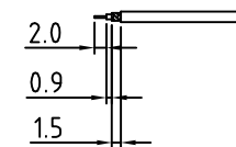
RECOMMENDED CABLE STRIPPING DIM
