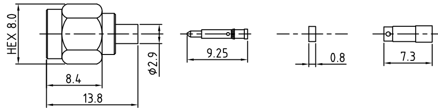
SMA ST PLUG DETAIL DIMENSION
