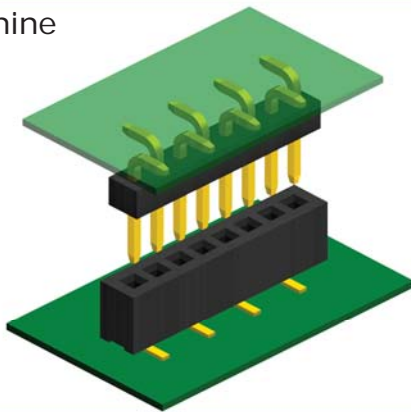
Mezzanine Stacking
