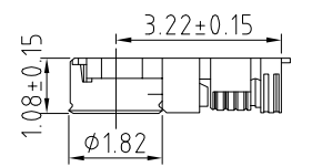
IPEX 4L PLUG DIMENSION
